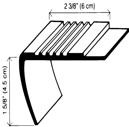
SN061 (STAIRNOSING)
